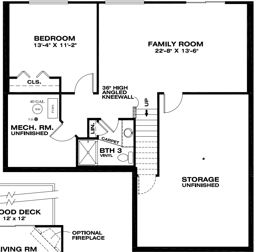
LOWER LEVEL FINISH OPTION 8' CEILING HT. ADDS 633 SF
